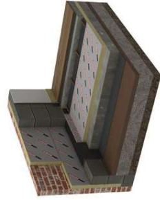
Above ground bearing slabs
