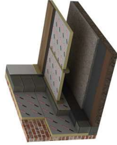
Suspended timber floor
