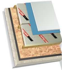
Timber wall mechanical fix
