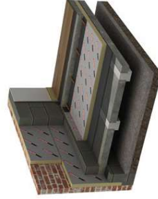
Beam & block detail
